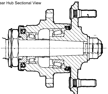
TR6 Rear Hub Sectional View
